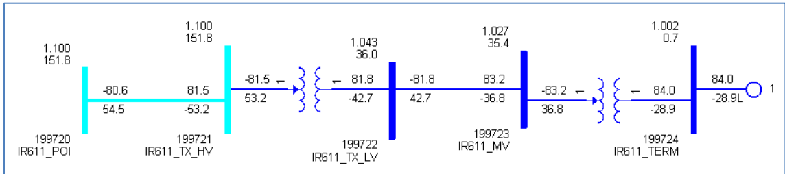
Figure 6 Power Factor with Qmin
